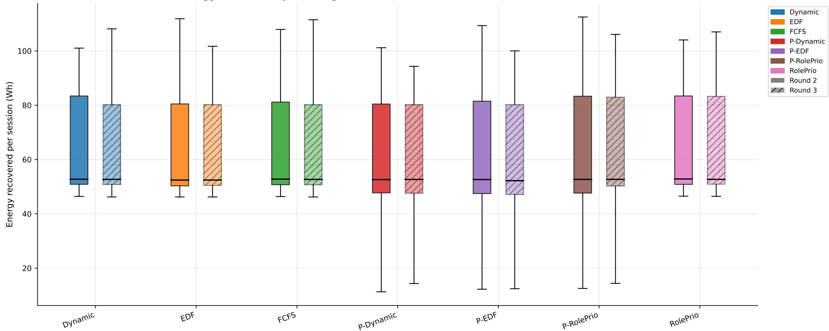
Energy Recovered per Charge Session — Round 2 (solid) vs Round 3 (hatched)
