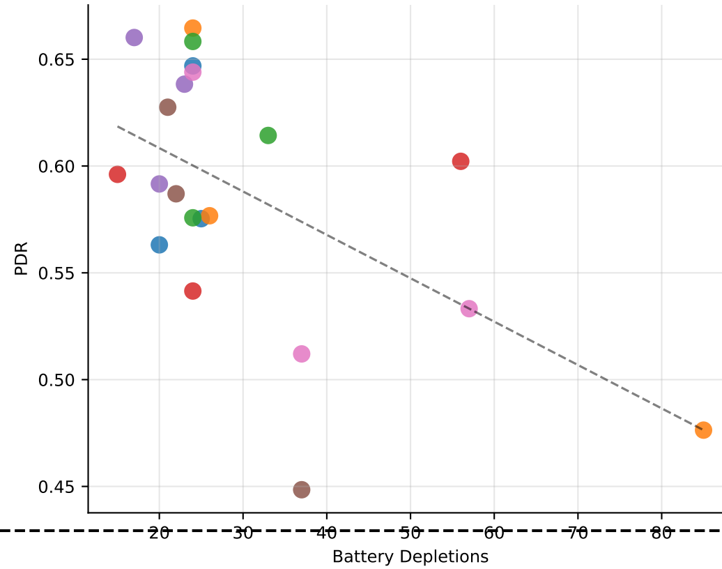
[Round 3] Fleet Survival → Network PDR r=-0.50, \rho=-0.28
