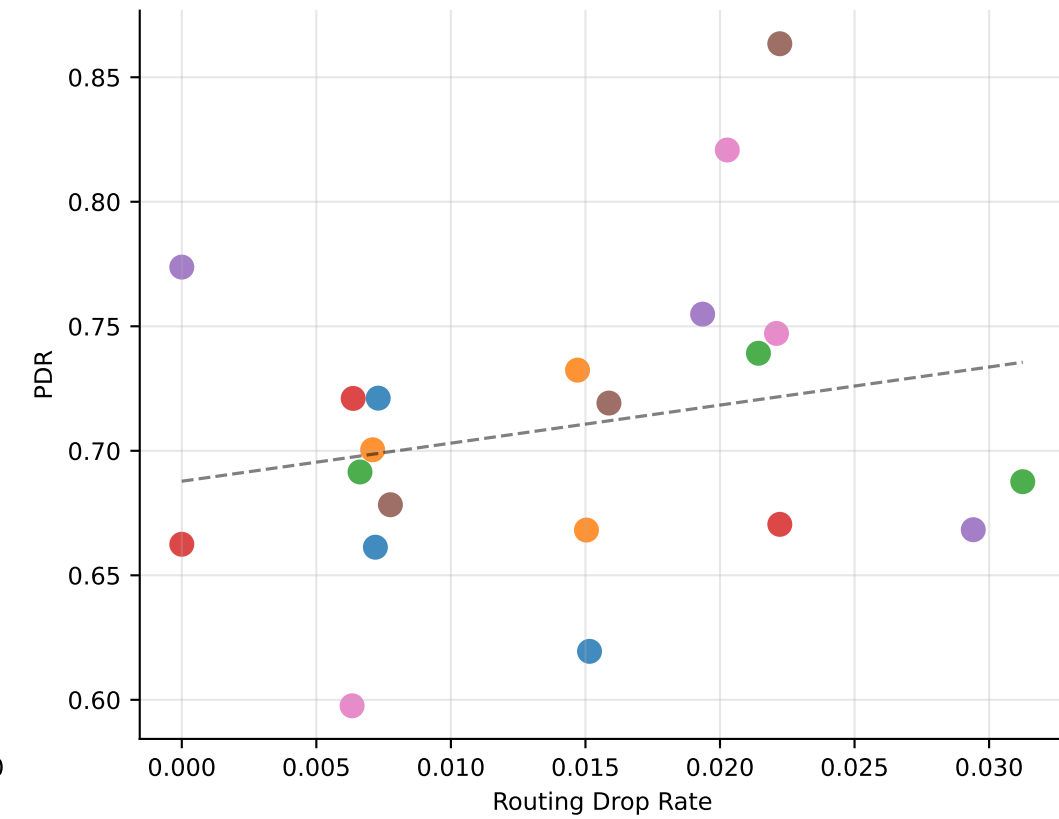
[Round 3] Routing Drops → Network PDR r=0.22, \rho=0.23
