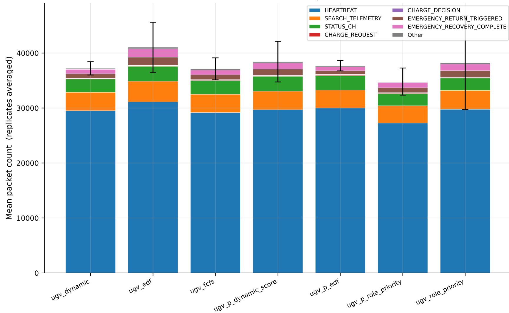
Packets Generated — Mean per Protocol
