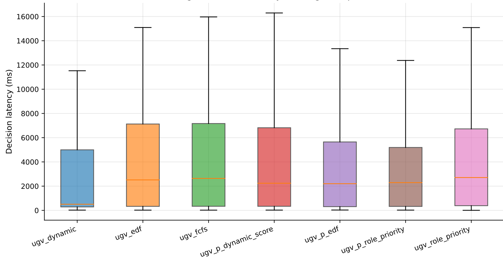
Charge Decision Latency — Merged Replicates
