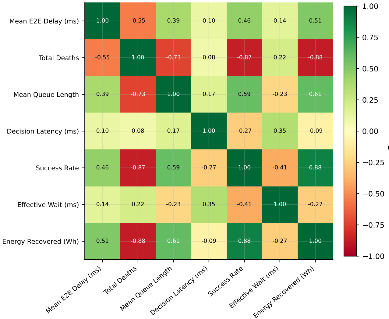
Pearson Correlation — Mean E2E Delay & Charging KPIs (per run)
