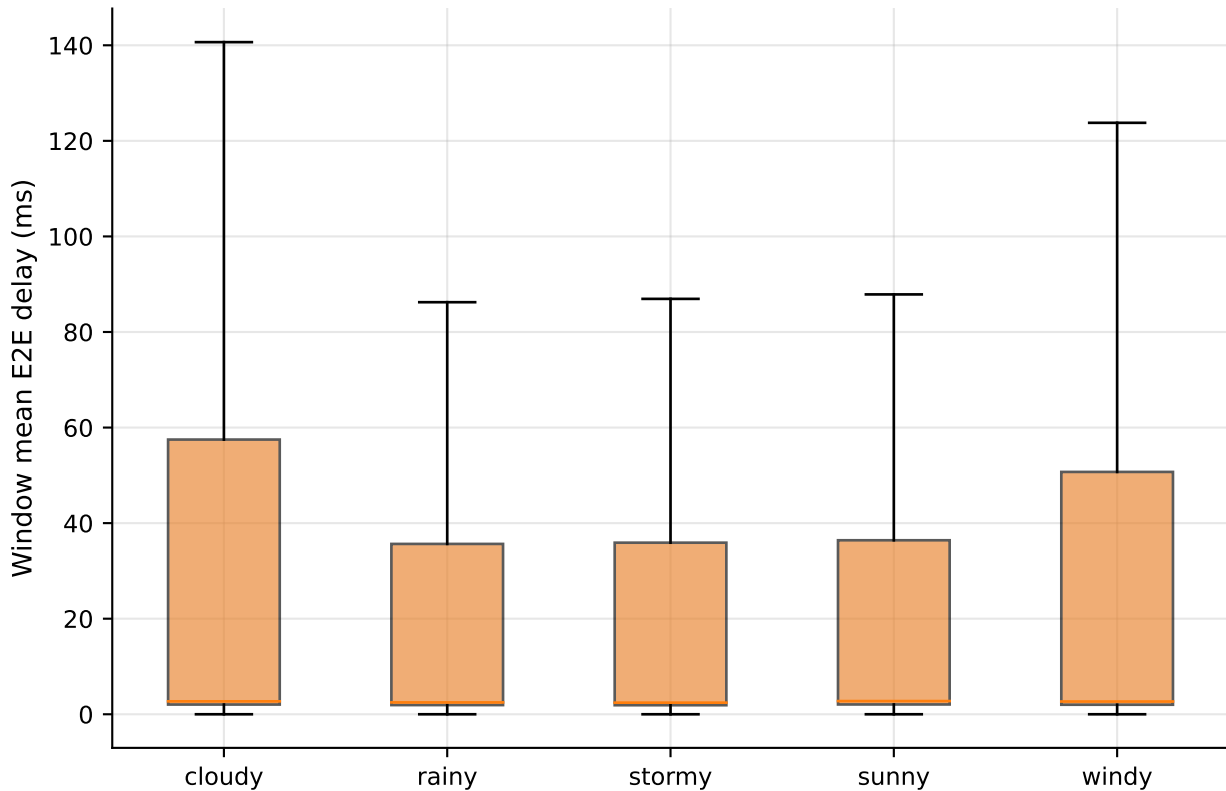
Message E2E Delay vs Weather Regime (all protocols)
