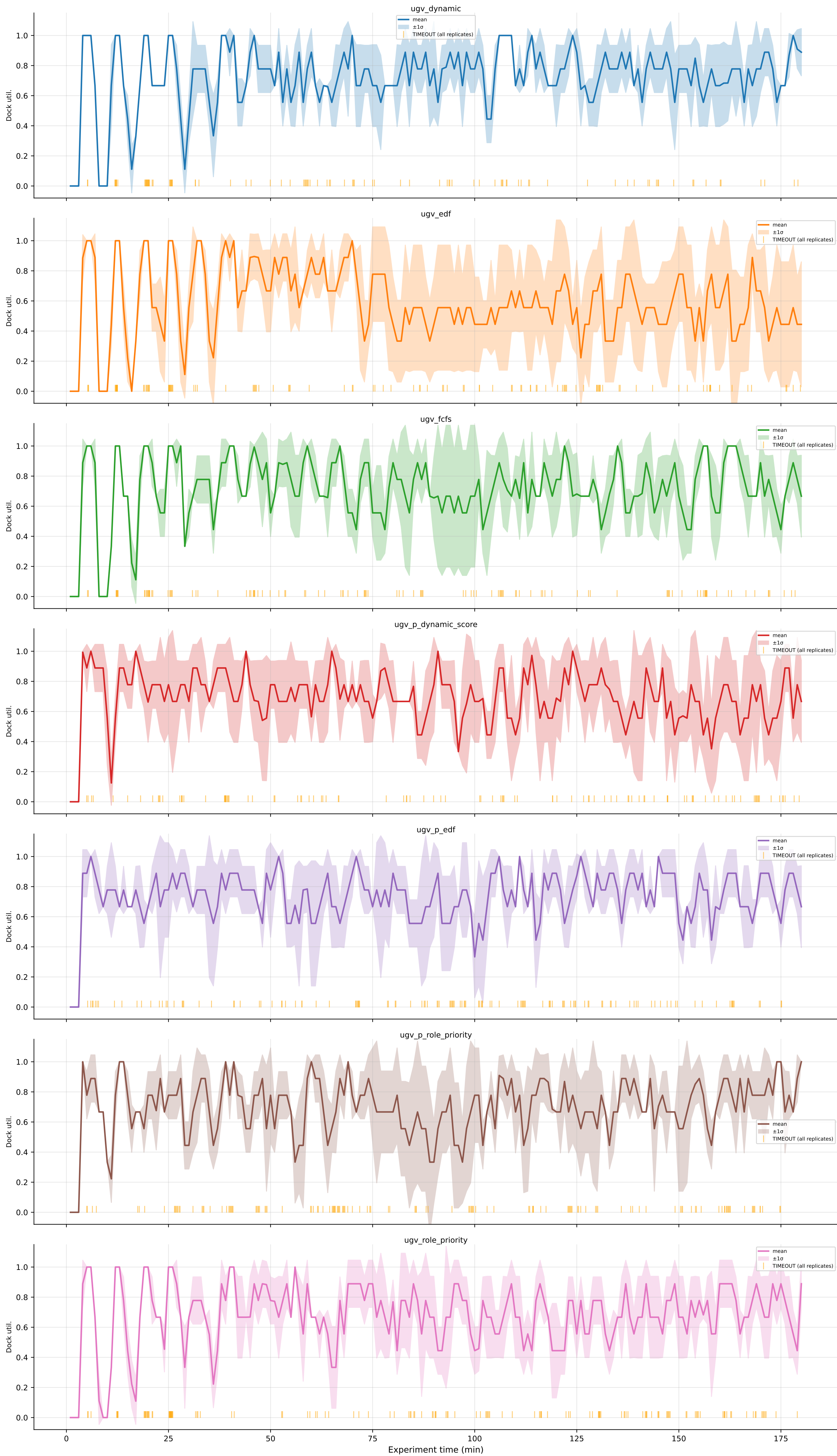
Dock Utilisation — Merged Replicates (mean \pm 1\sigma ) + TIMEOUT Events
