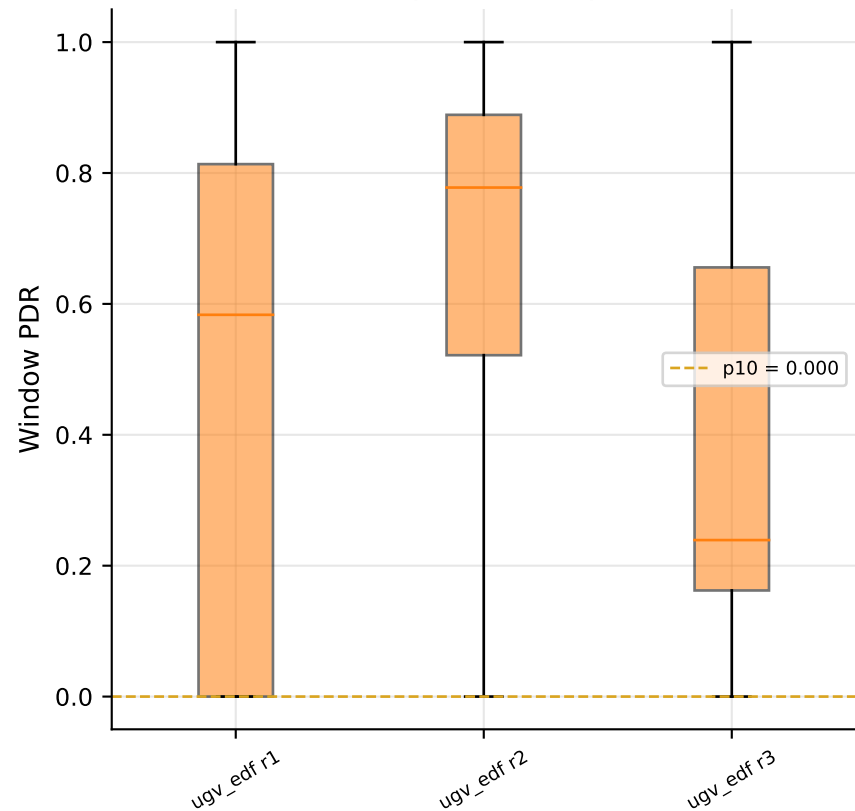
Per-replicate boxplot
