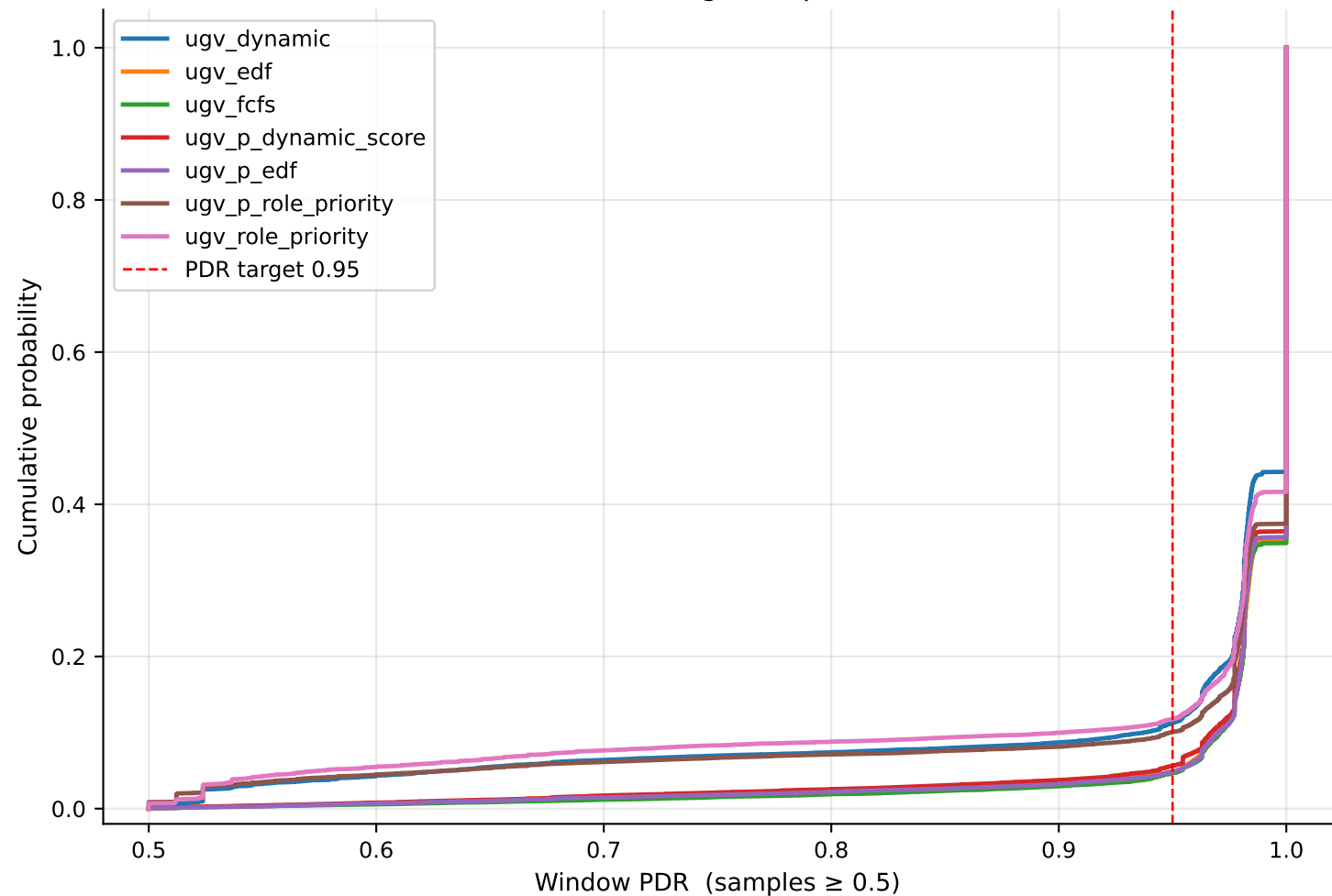
Network PDR CDF — Merged Replicates (PDR \geq 0.5 )
