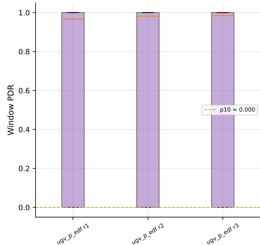
Per-replicate boxplot
