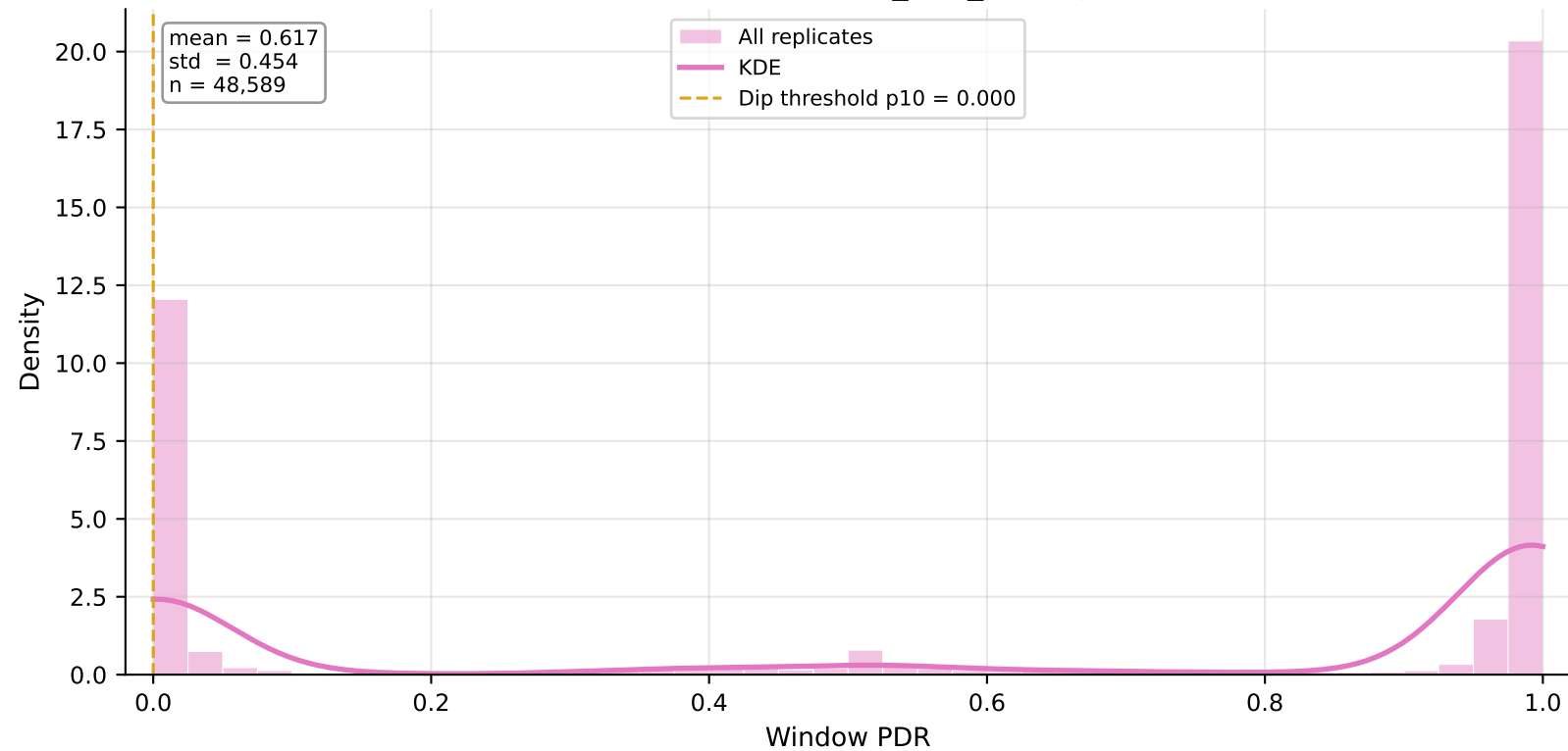
Distribution — ugv_role_priority
