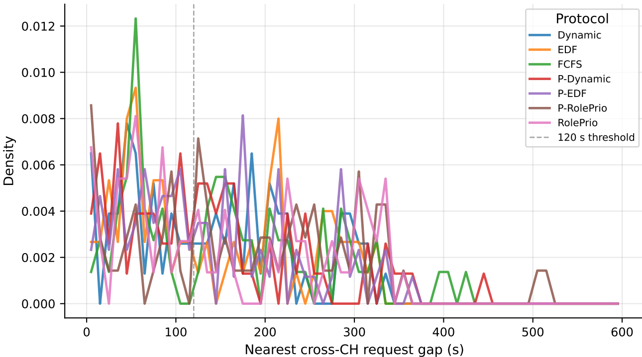
CH Request Temporal Proximity (all protocols: CHs deplete in sync due to identical battery capacity)
