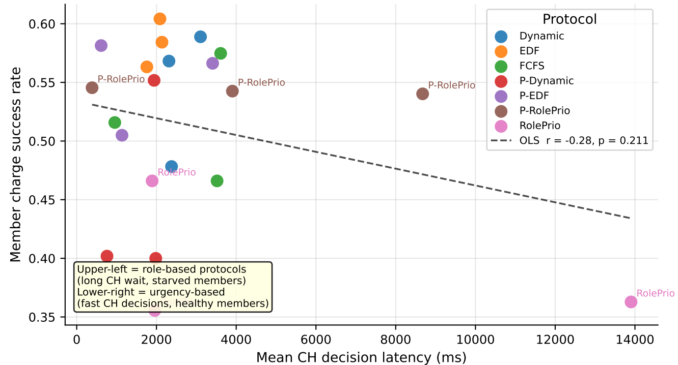
CH Wait Time vs Member Success Rate (role-based: long CH wait → member starvation)
