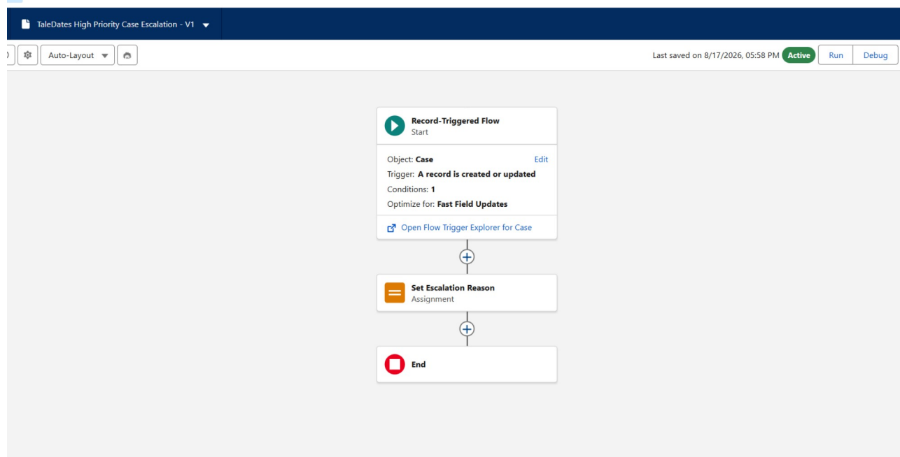
Figure 21. Active record-triggered High Priority Case Escalation Flow.
