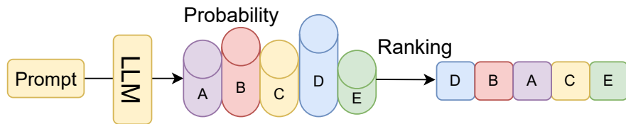
(B) Single Token Generation (e.g., FIRST)
