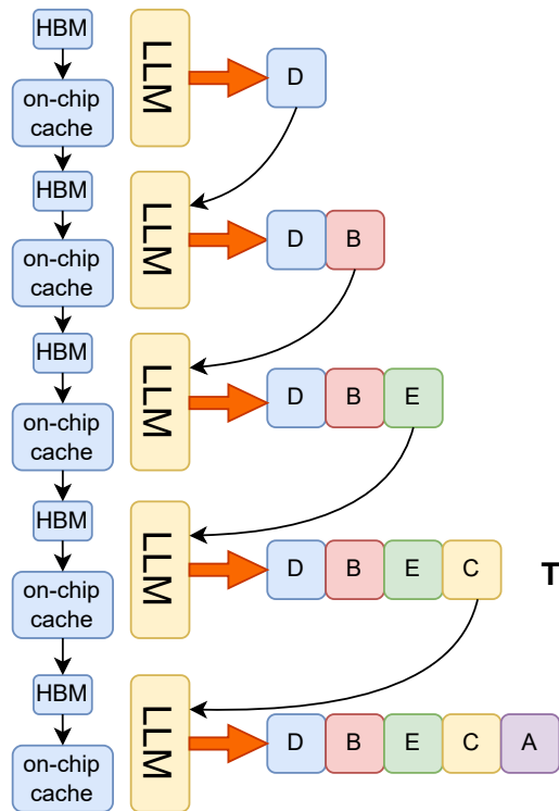
(A) Auto-regressive generation
