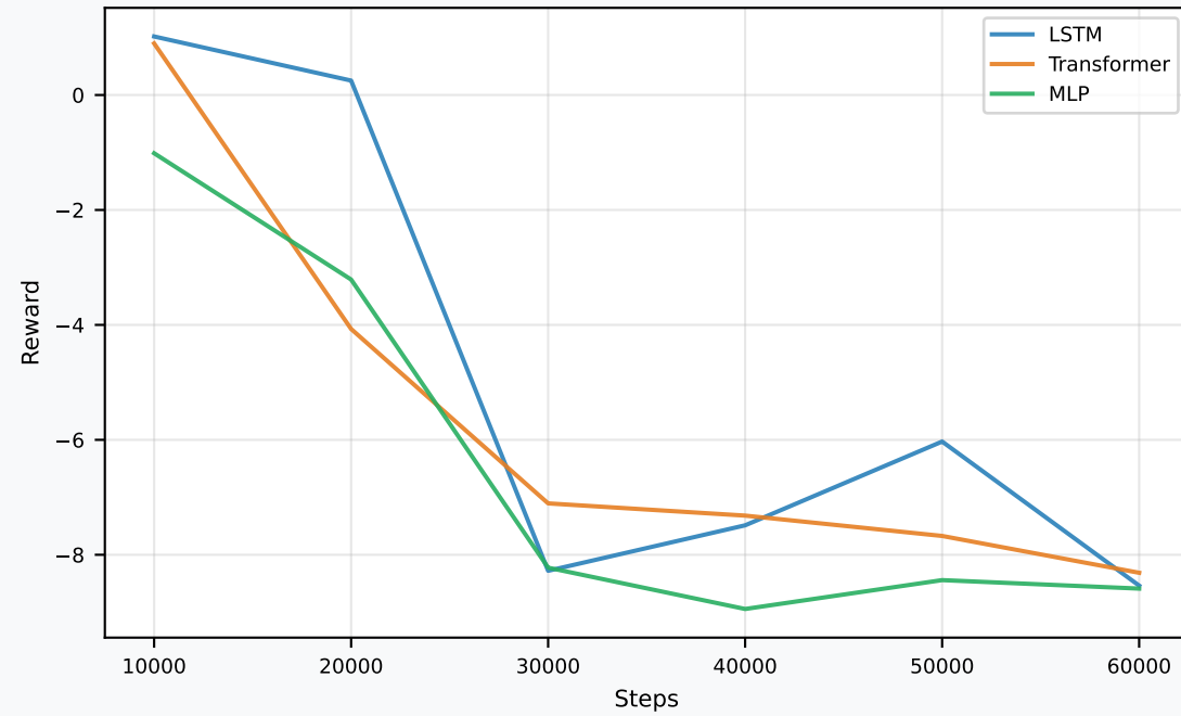
Curriculum Phase
