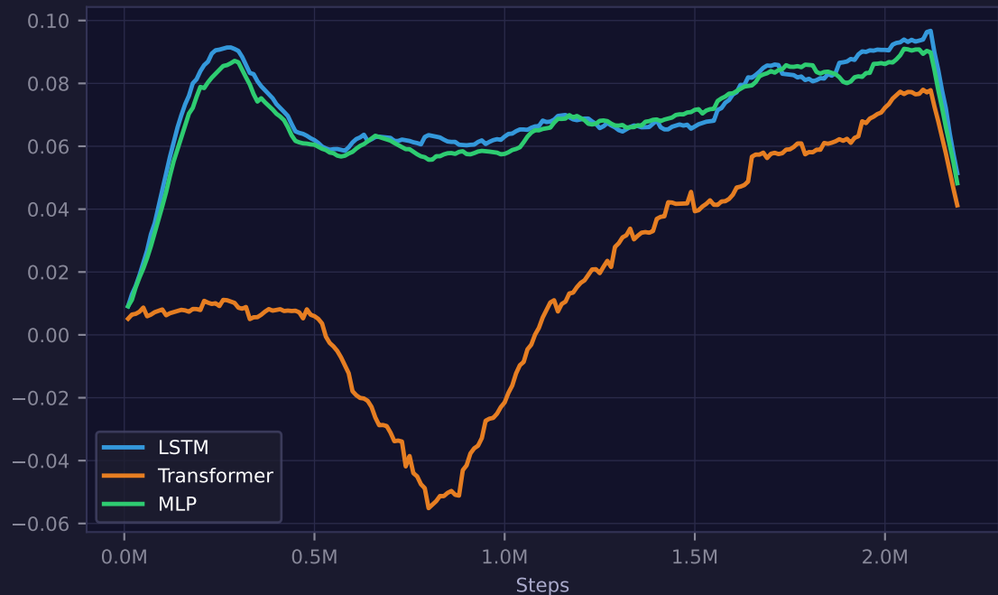
Curiosity Reward
