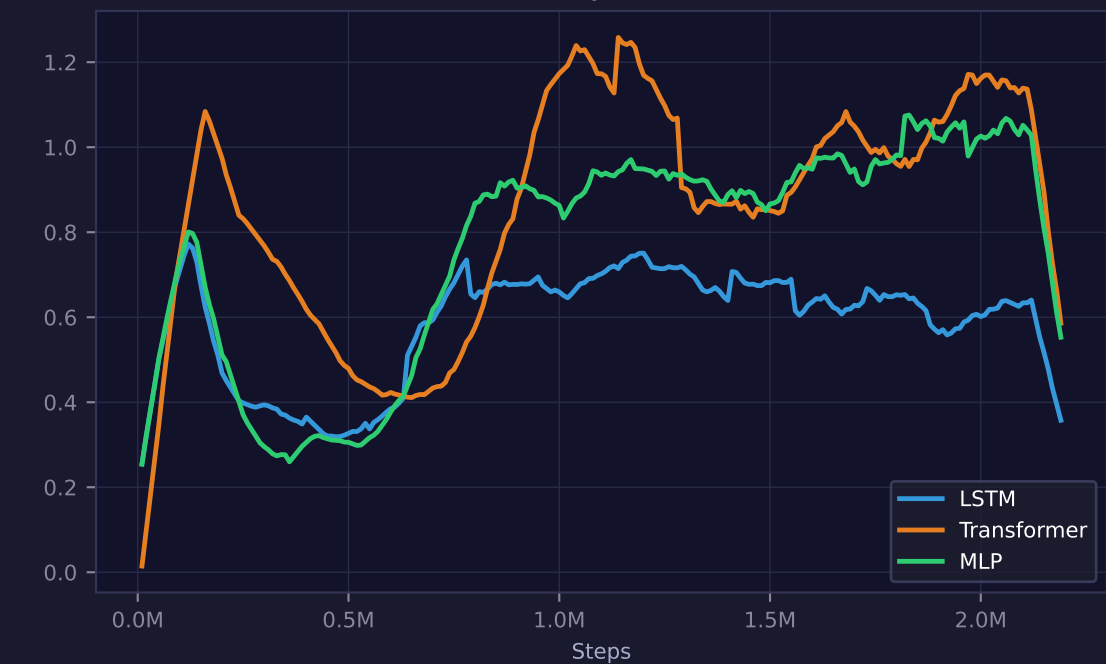
Curiosity Reward
