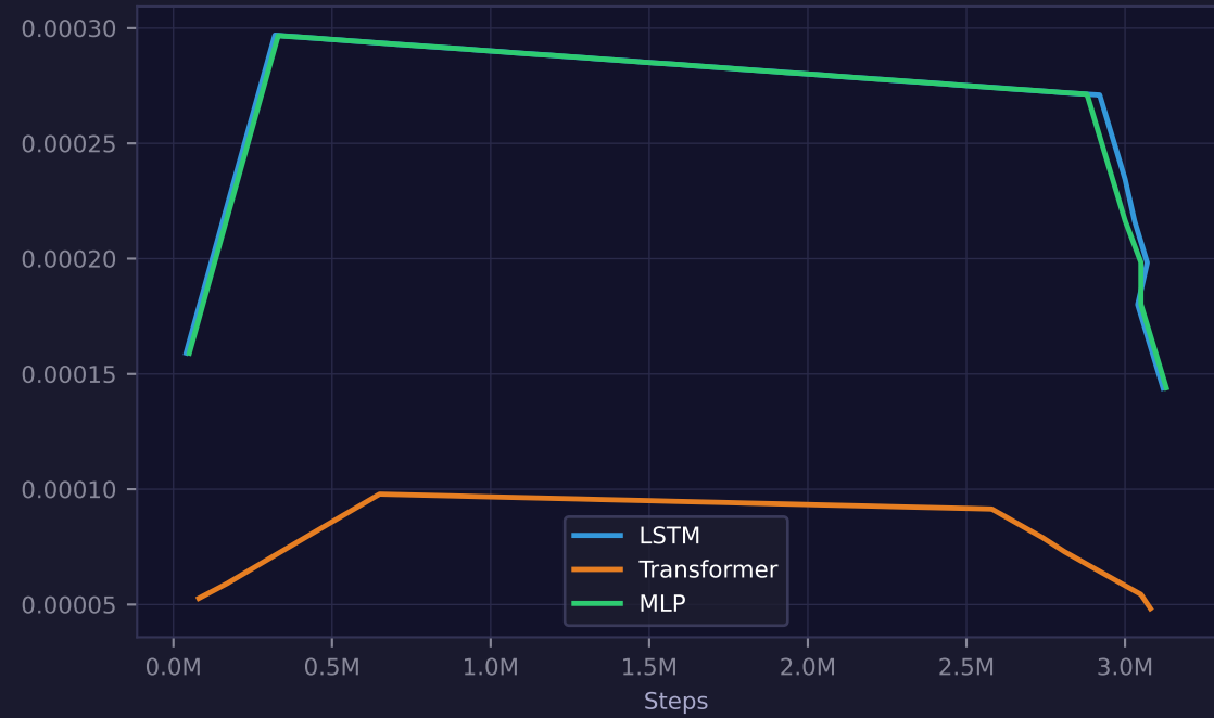
Learning Rate
