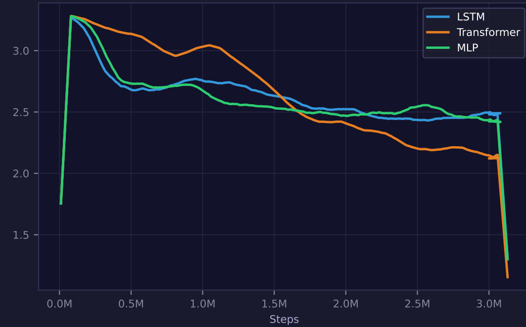
Entropy
