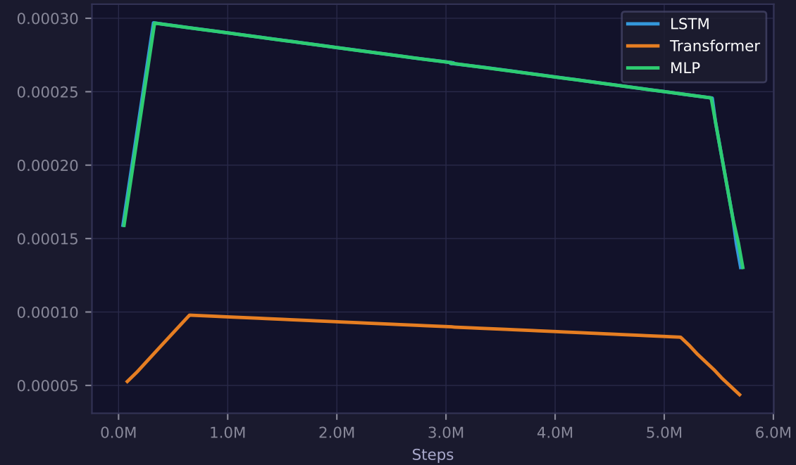
Learning Rate
