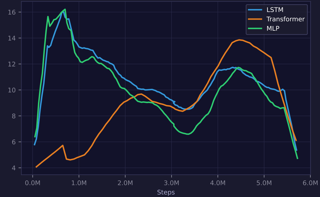
Learning Rate
