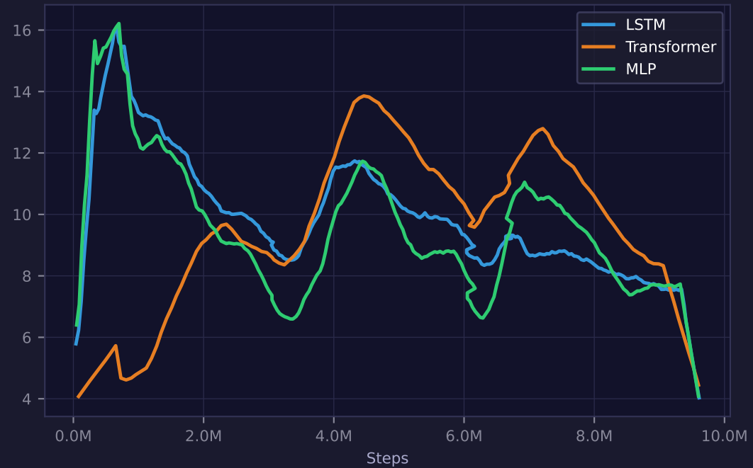
Learning Rate
