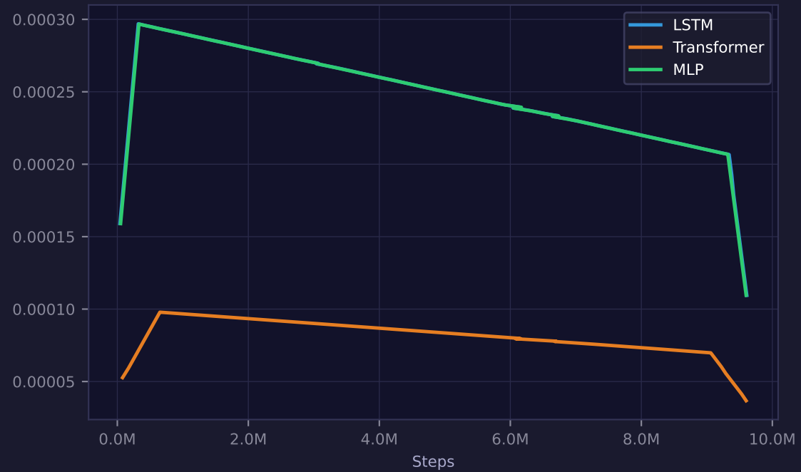
Learning Rate
