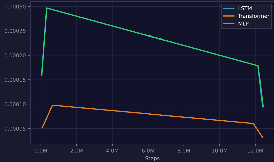
Learning Rate
