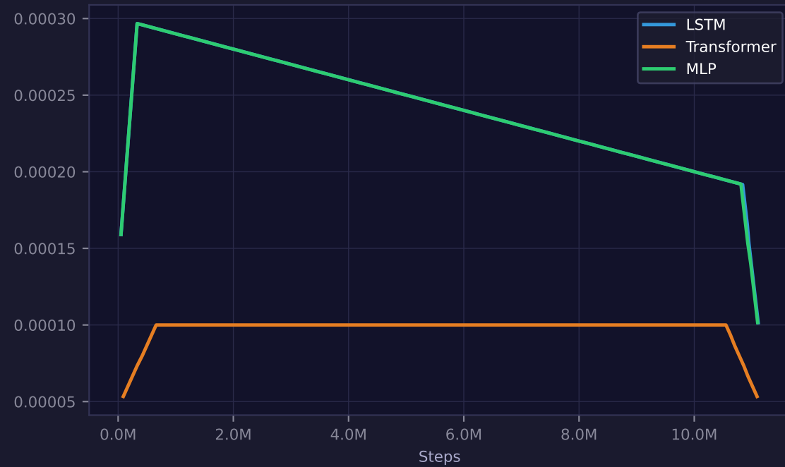
Learning Rate
