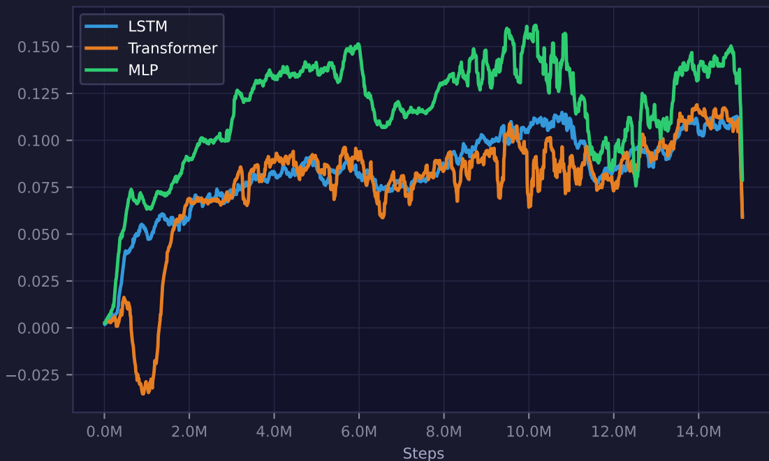
Curiosity Reward
