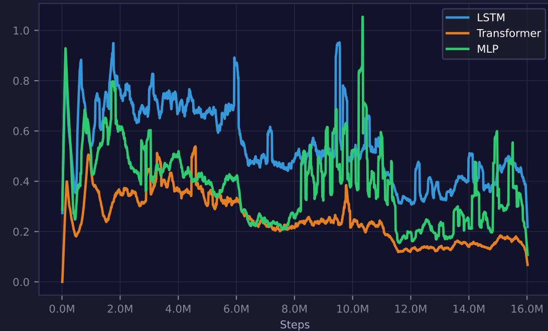
Curiosity Reward
