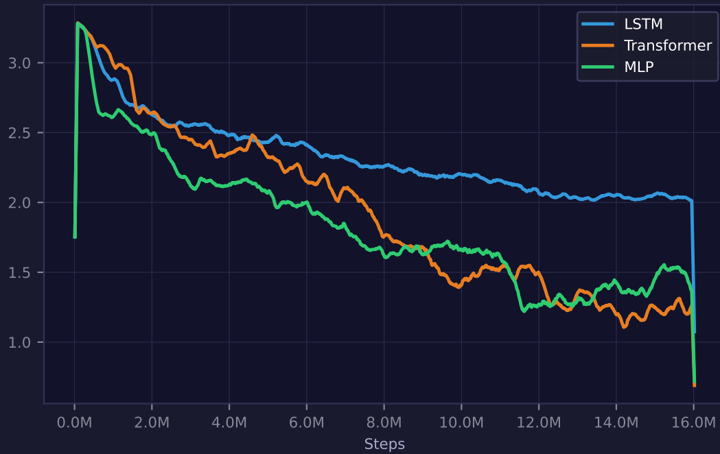
Entropy
