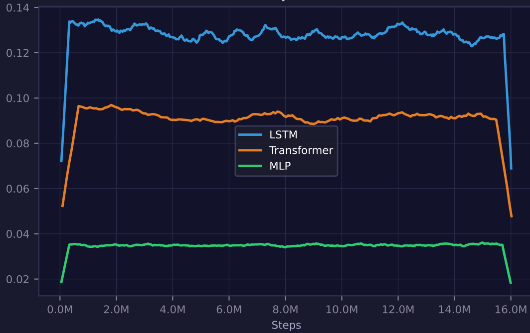
Entropy
