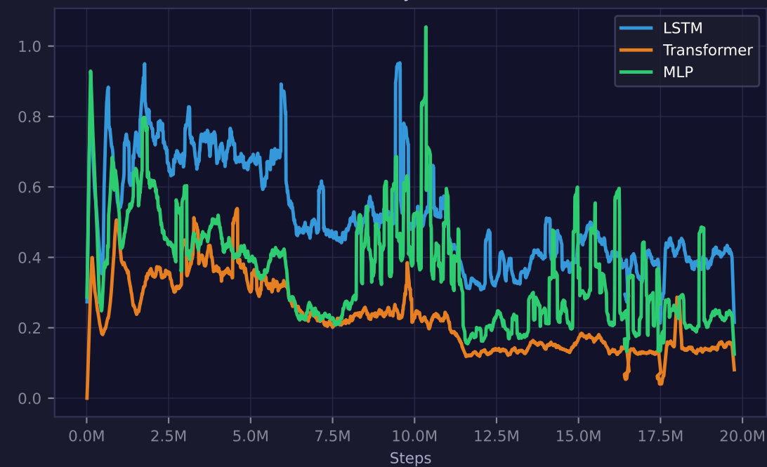
Curiosity Reward
