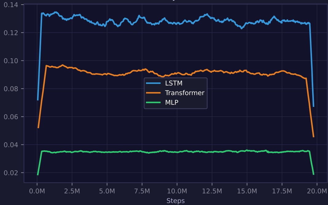
Entropy
