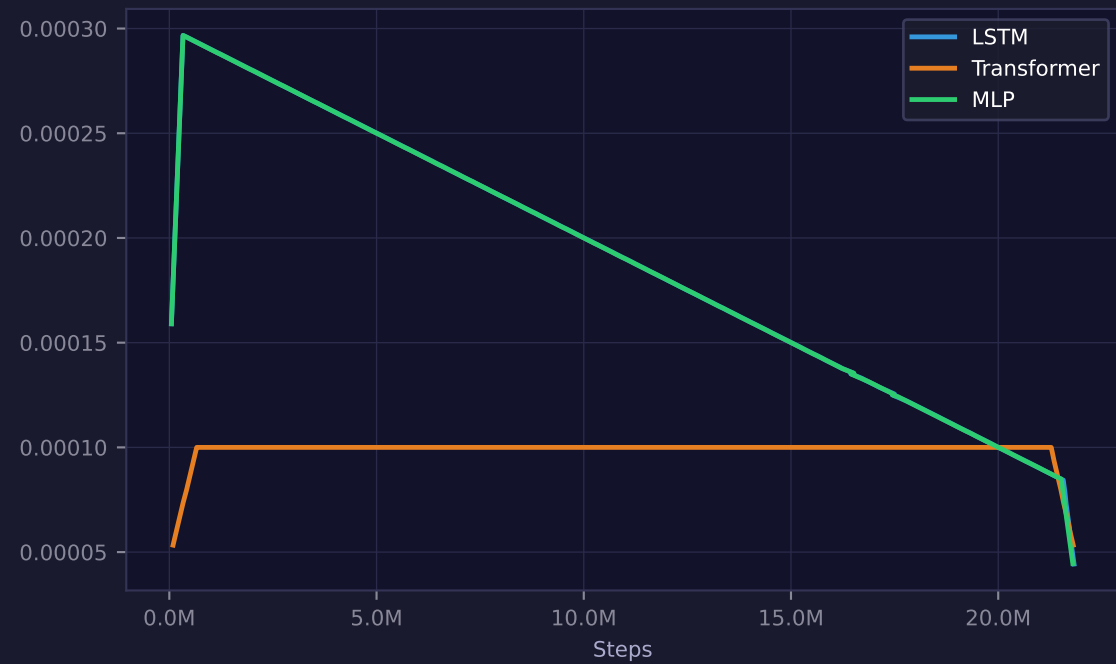
Learning Rate
