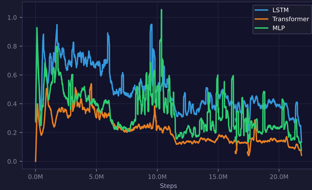
Curiosity Reward
