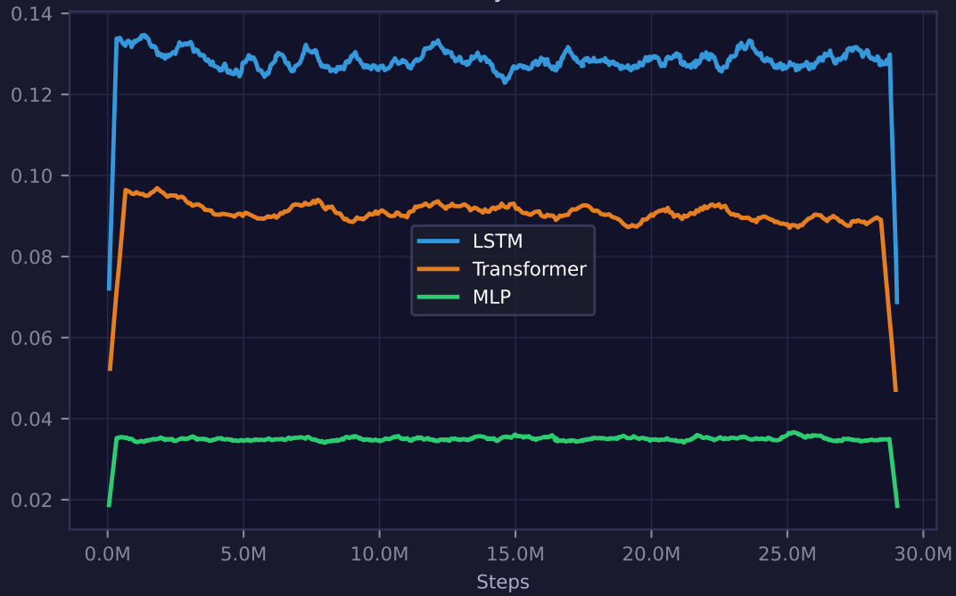
Entropy
