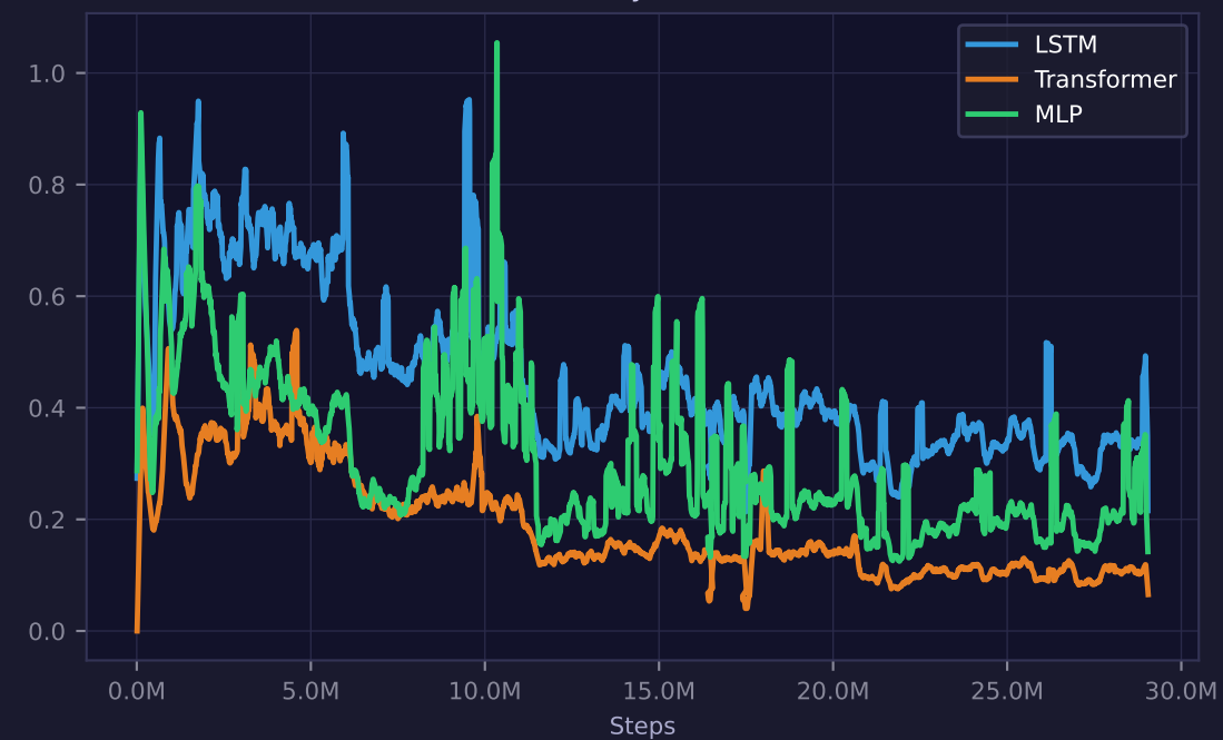
Curiosity Reward
