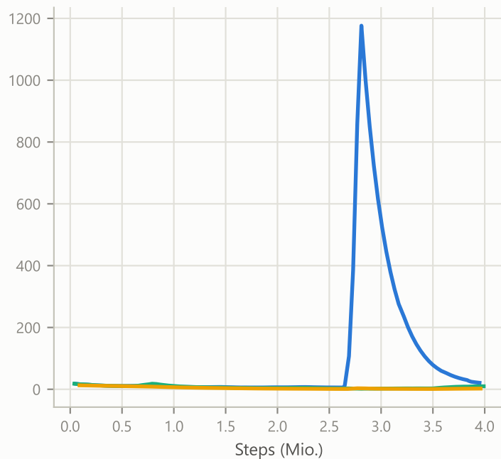
Value Loss
