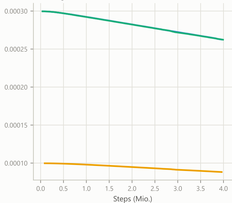
Learning Rate
