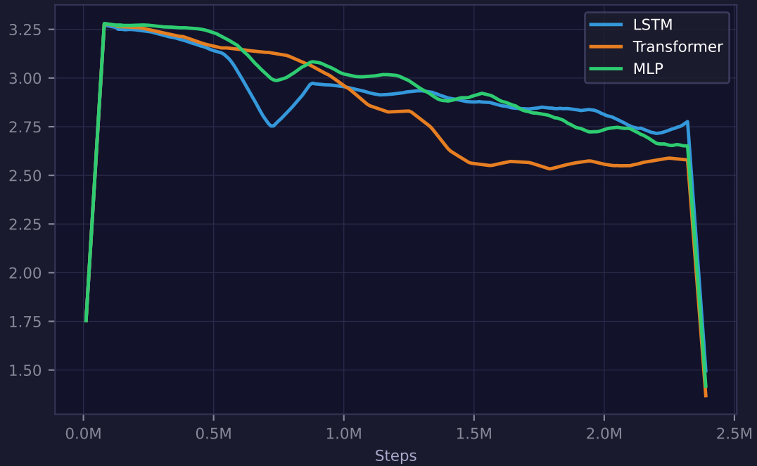
Entropy
