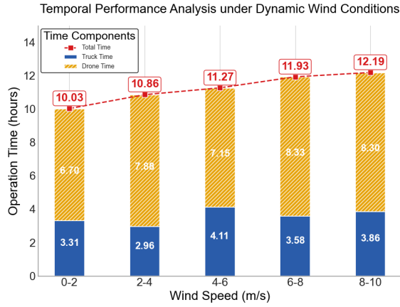
Fig. 16. Time variation diagram of multi-wind speed gradient UAVs and truck.
