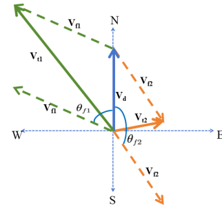
Fig. 3. UAV speed variation map.
