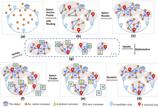
Fig. 4. ACLA process for handling dynamic customer demands.
