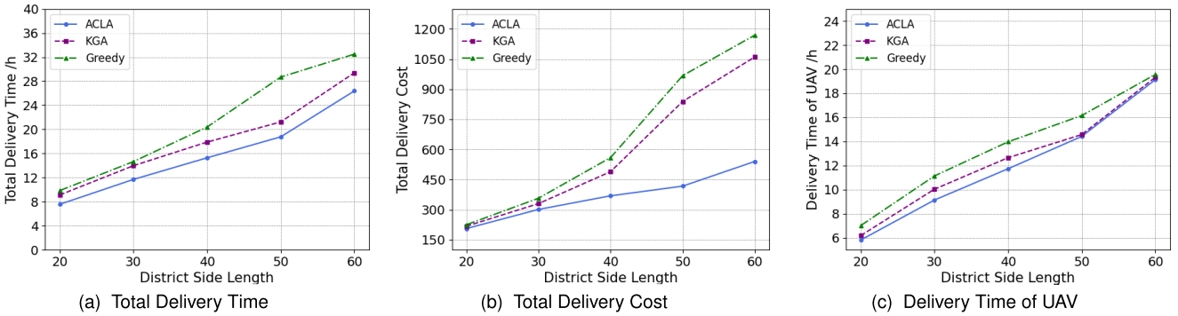
Fig. 10. The impact of different service area size.
