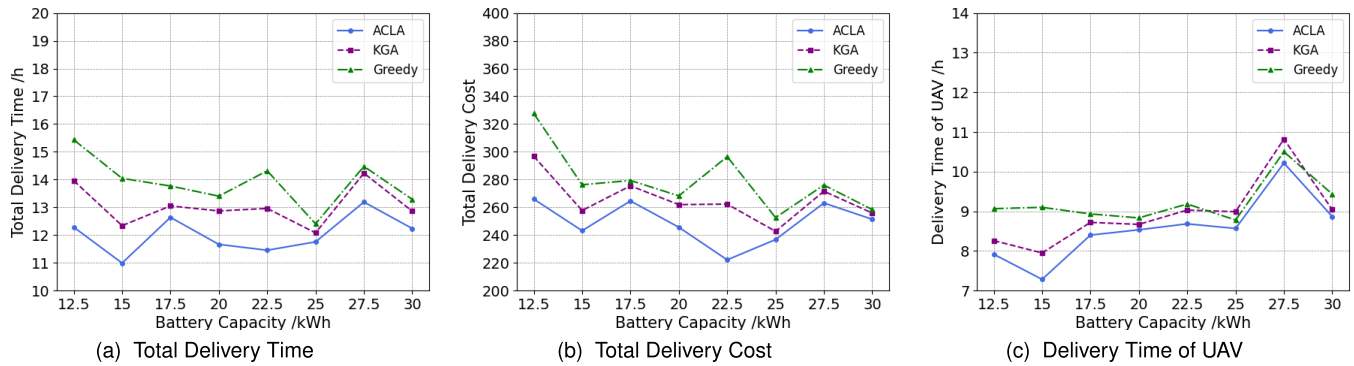
Fig. 13. The impact of different UAV battery capacity.
