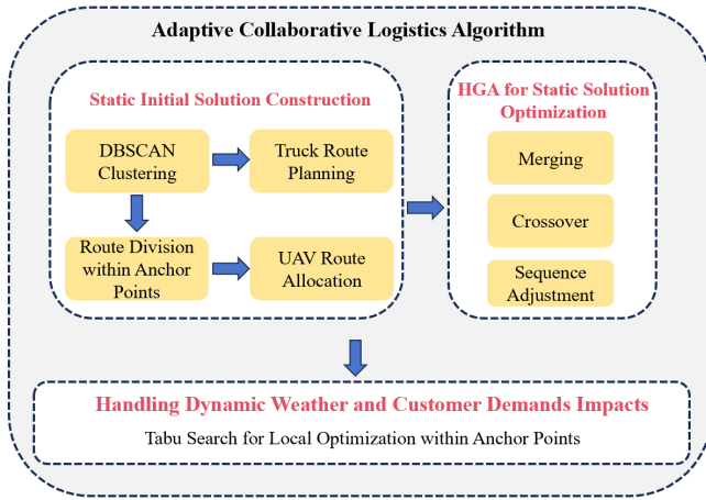
Fig. 5. Flowchart of the ACLA.
