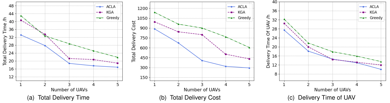
Fig. 11. The impact of different UAV numbers.
