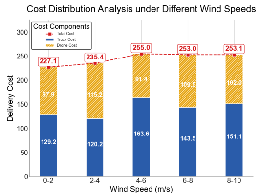
Fig. 15. Cost variation diagram of multi-wind speed gradient UAVs and truck.
