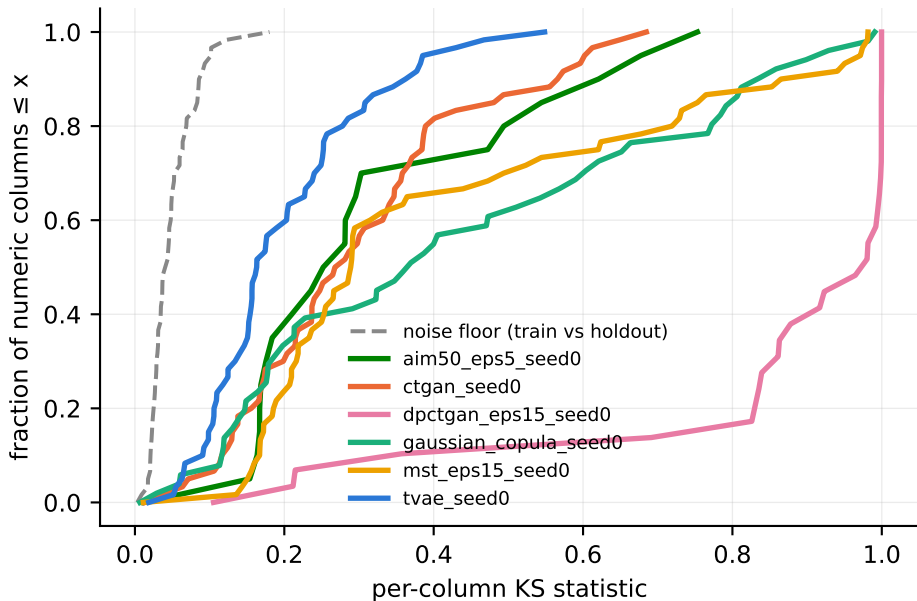
Numeric fidelity profile vs the sampling-noise floor
