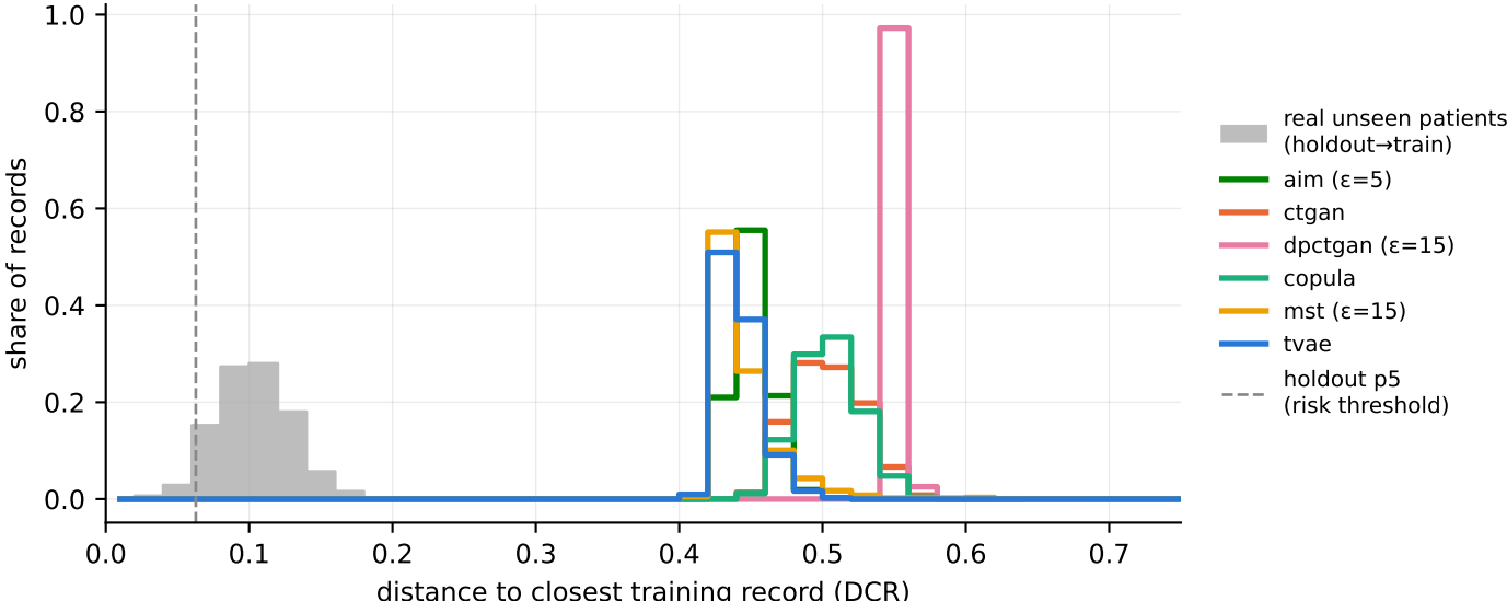
Privacy: synthetic records vs the unseen-patient baseline
