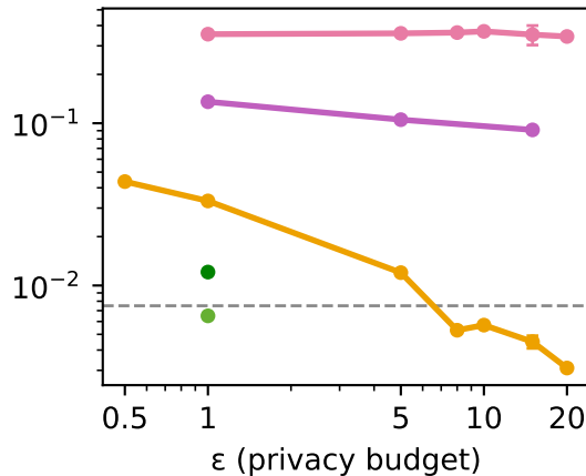
missingness MAD
