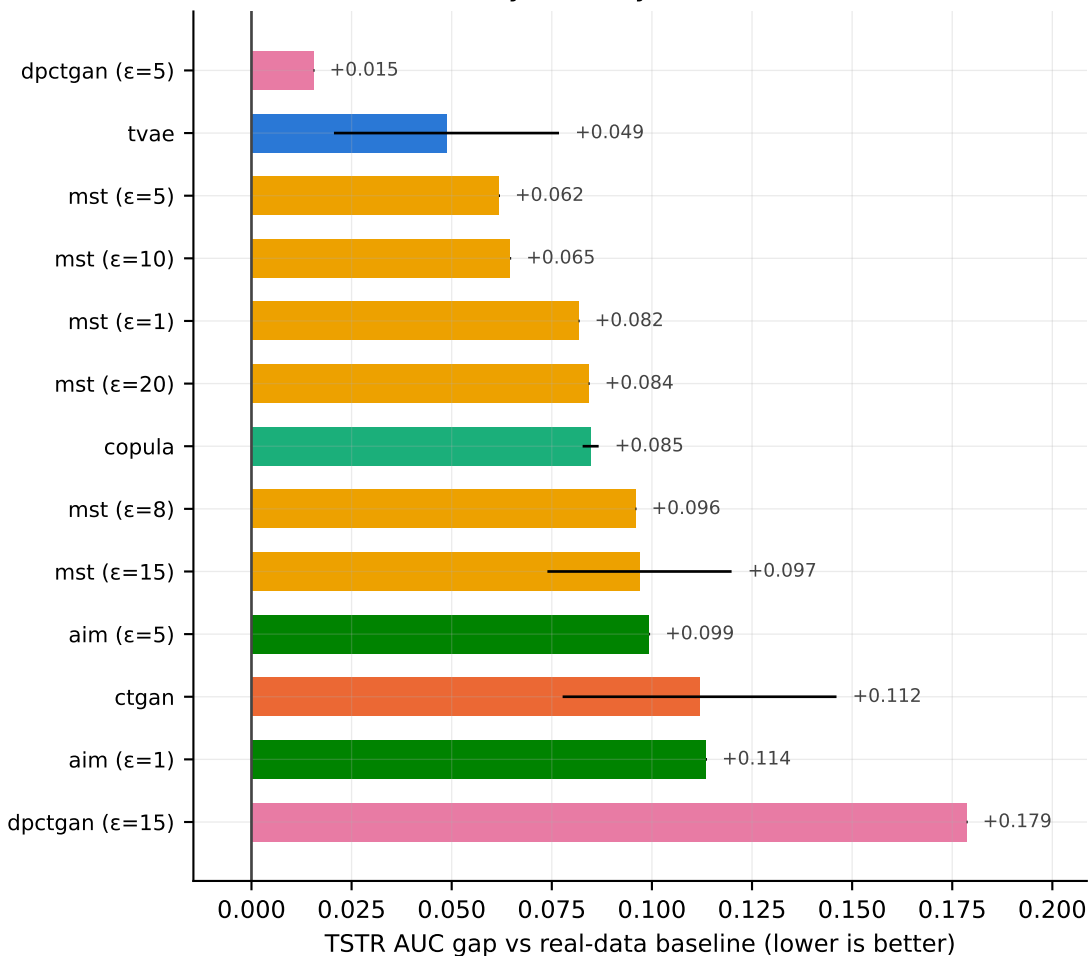
Downstream utility: train-synthetic, test-real (holdout)
