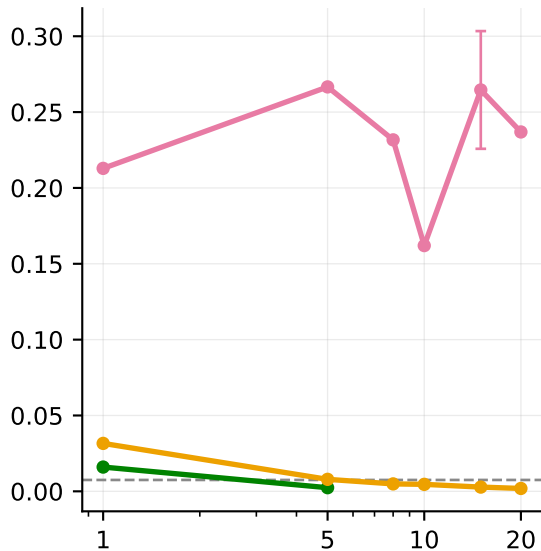
missingness MAD
