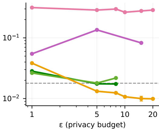
TVD mean (categorical)
