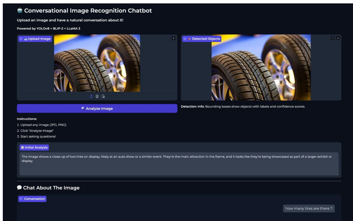
Figure C.1 Initial Image Upload and Scene Analysis
