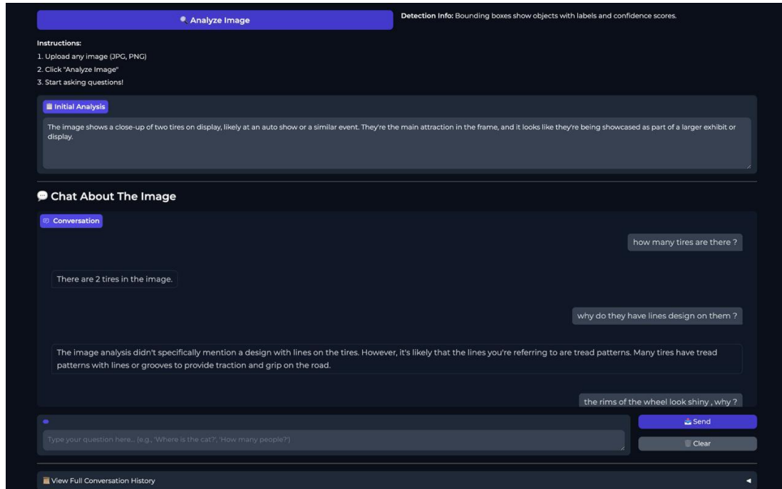
Figure C.2 Conversational Response – Object Count
