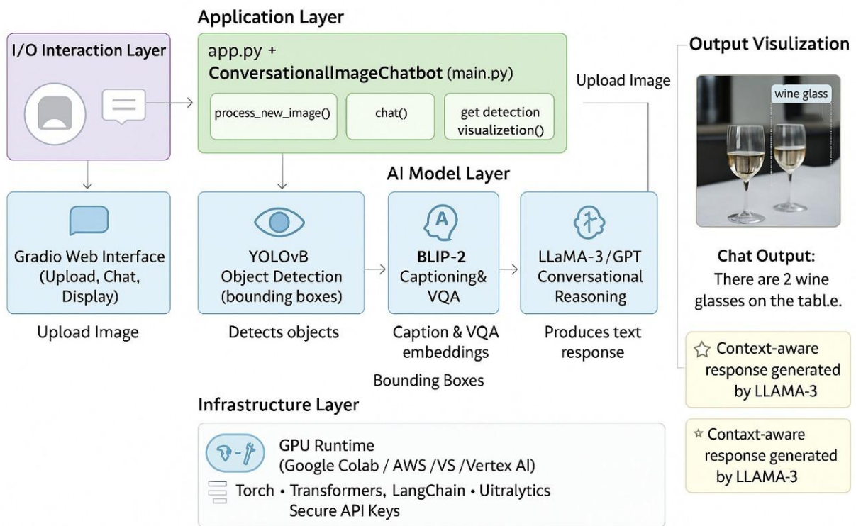
Figure 5.1 Architecture of Conversational Image Recognition Chatbot
