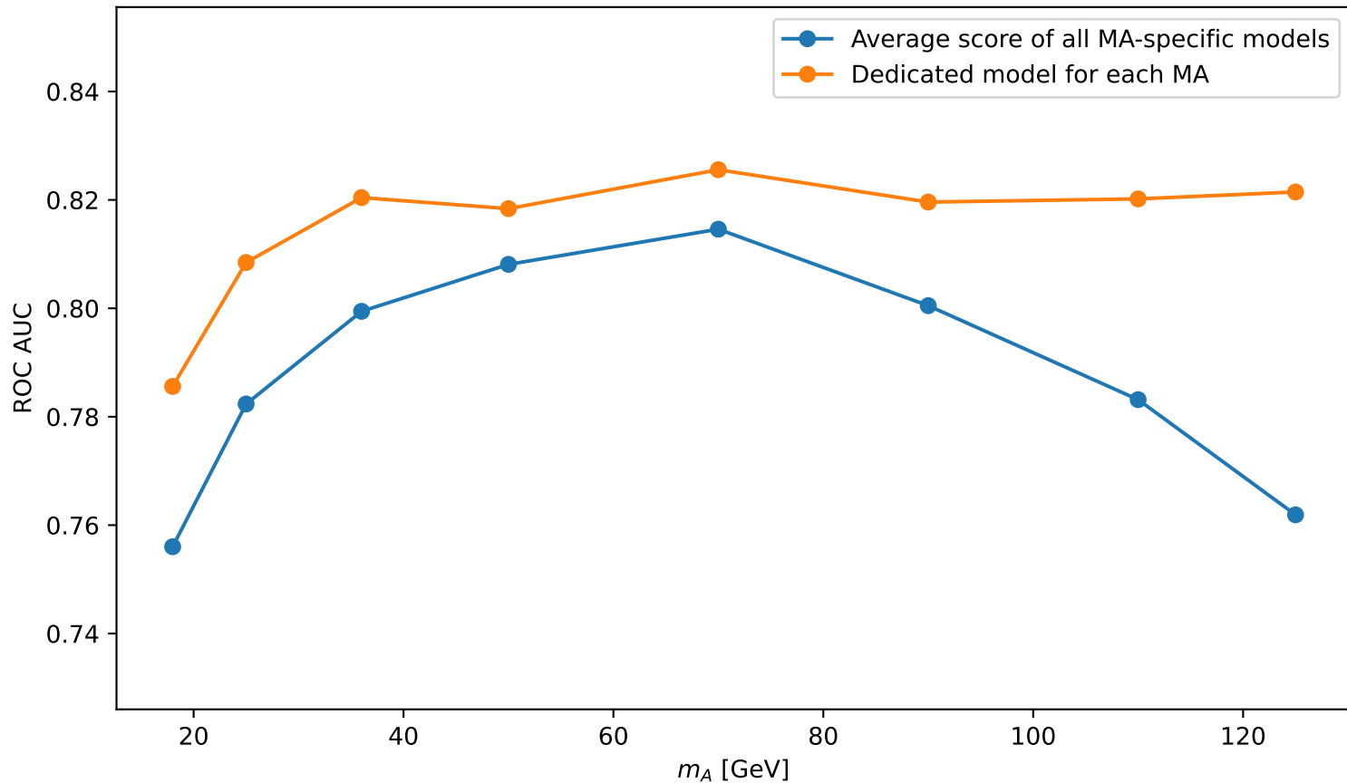
MA-specific ONNX evaluation (MHc=130 GeV)
