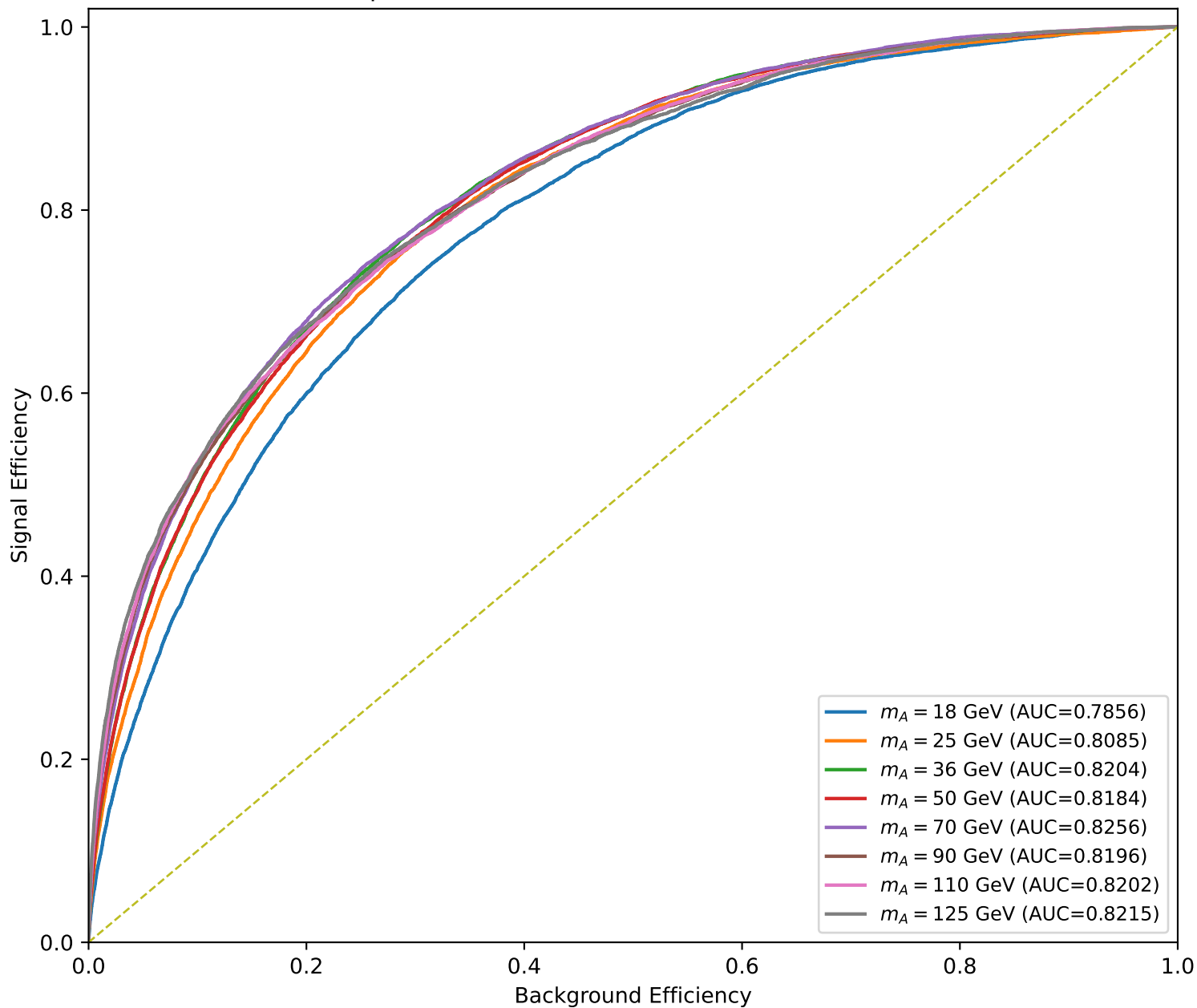
MA-specific ONNX: dedicated model for each mass
