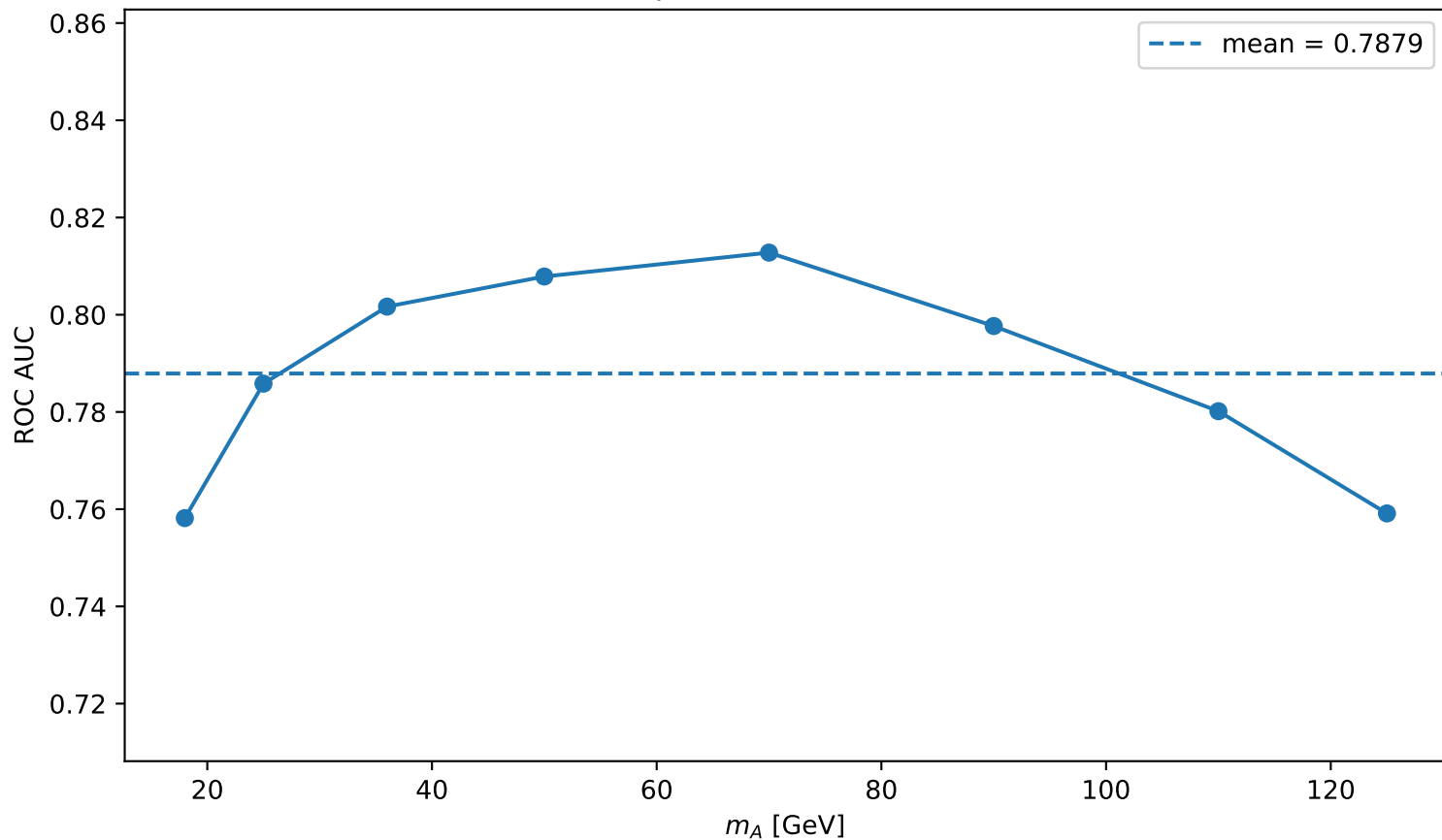
Combined-MA model performance vs mass (MHc=130 GeV)
