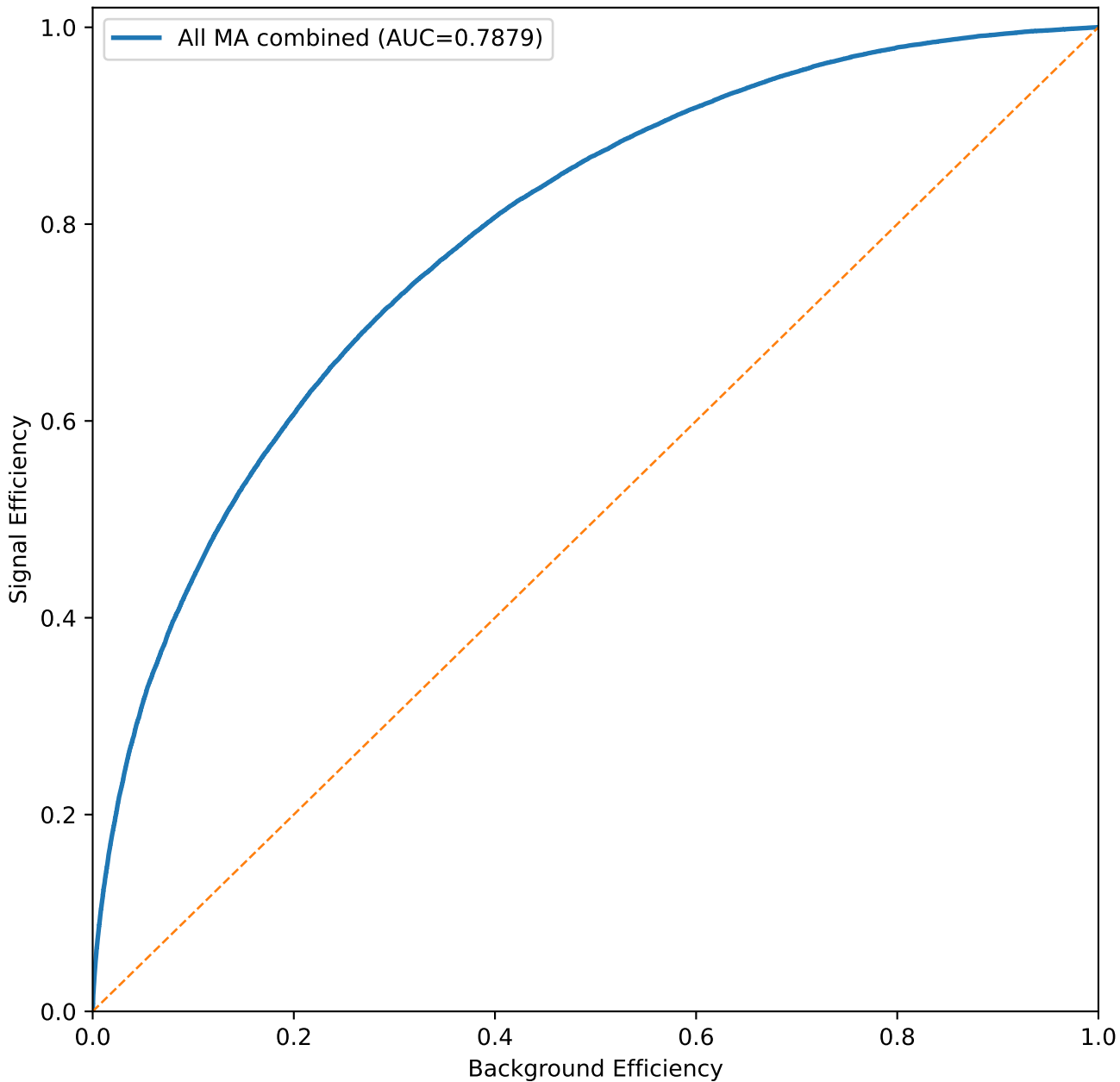
Combined-MA ONNX: all masses, M_{Hc}=130 GeV
