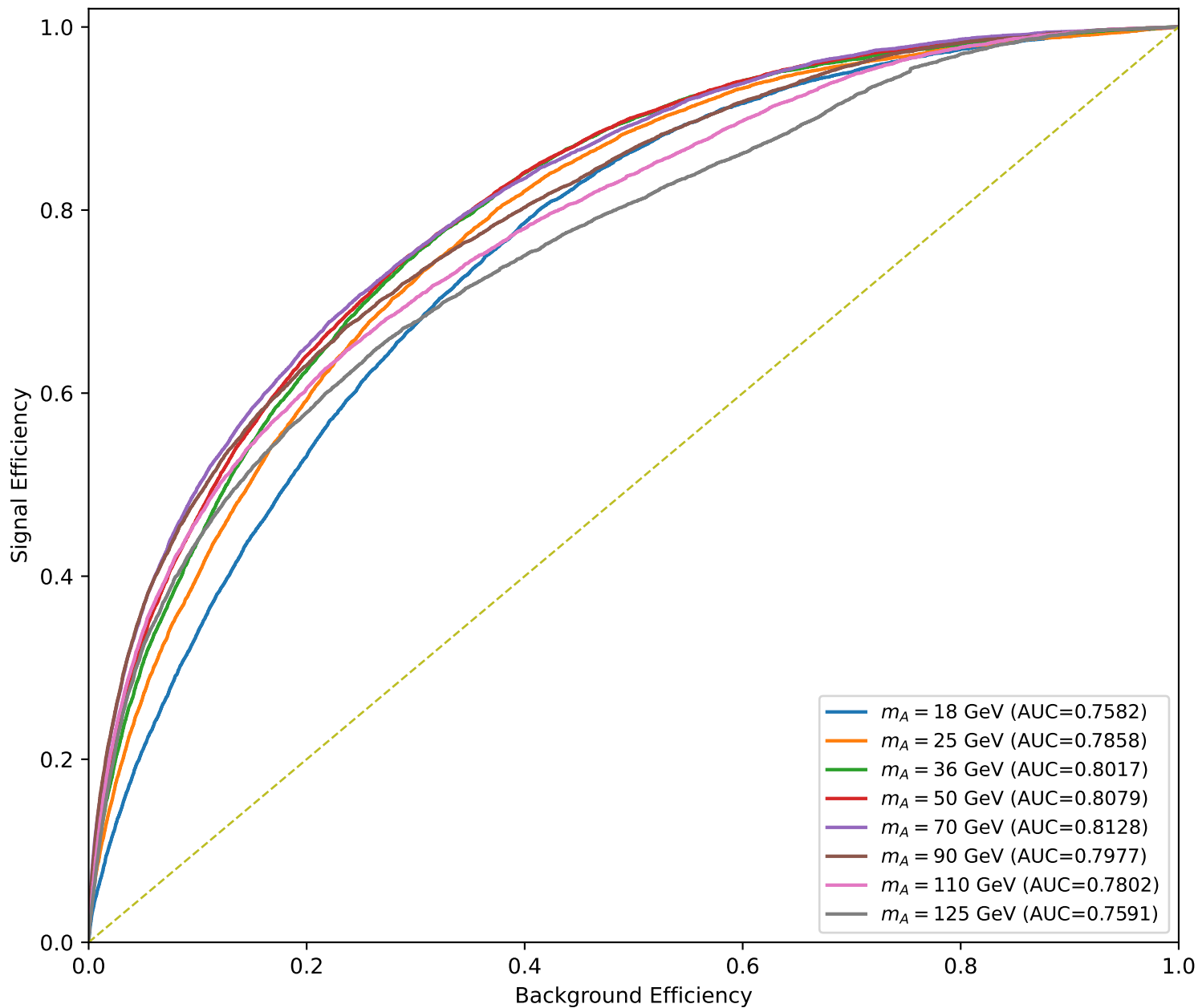
Combined-MA model: each mass, M_{Hc}=130 GeV
