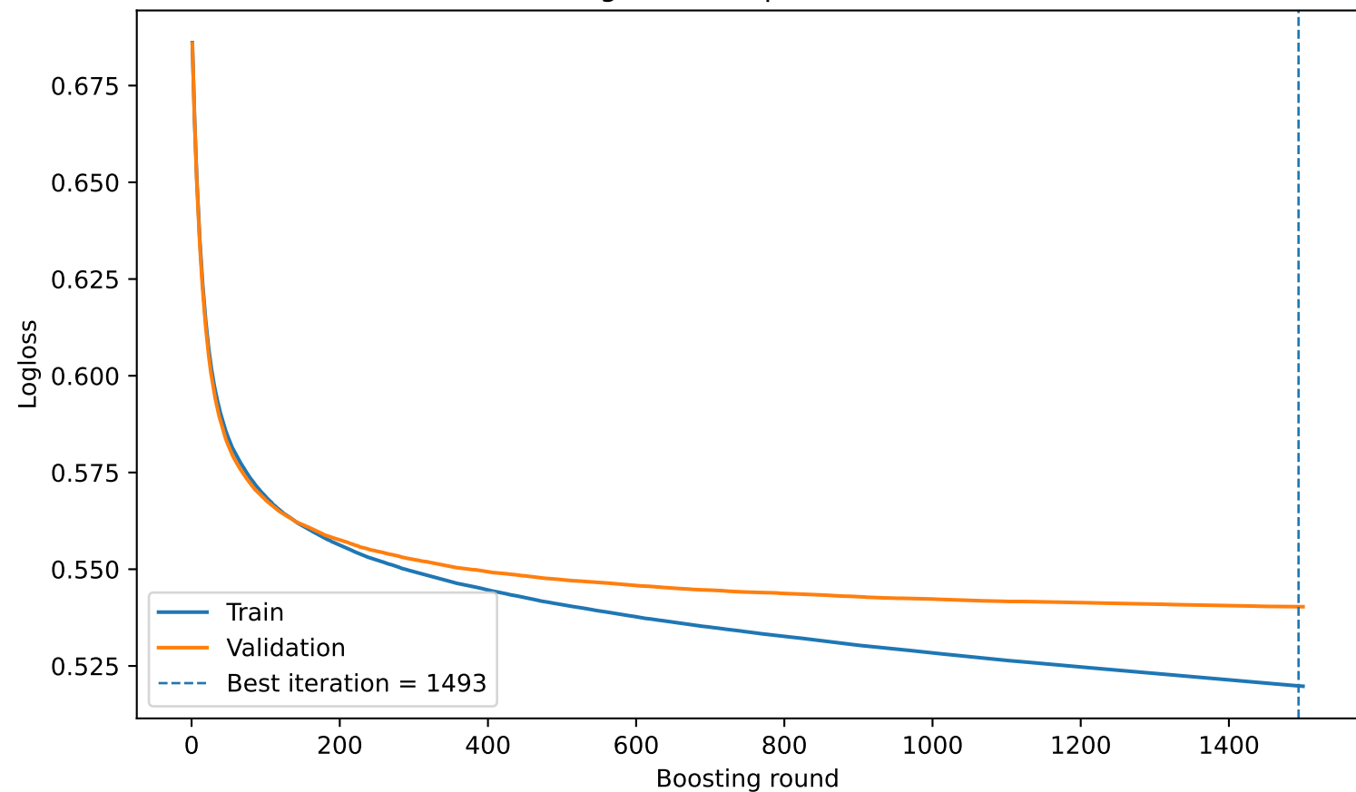
Learning curve: depth=3, child=30
