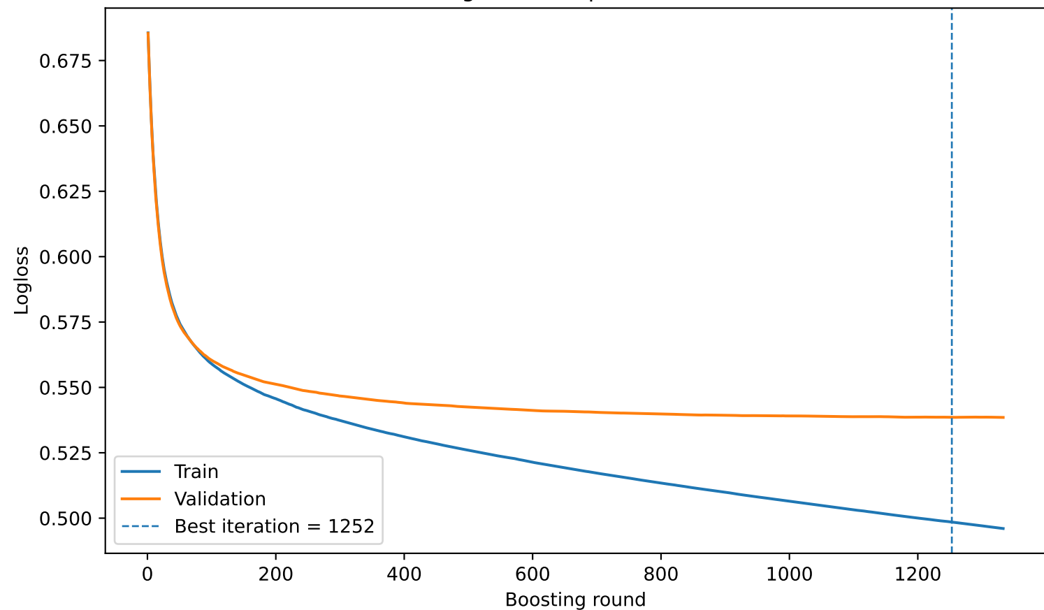
Learning curve: depth=4, child=10
