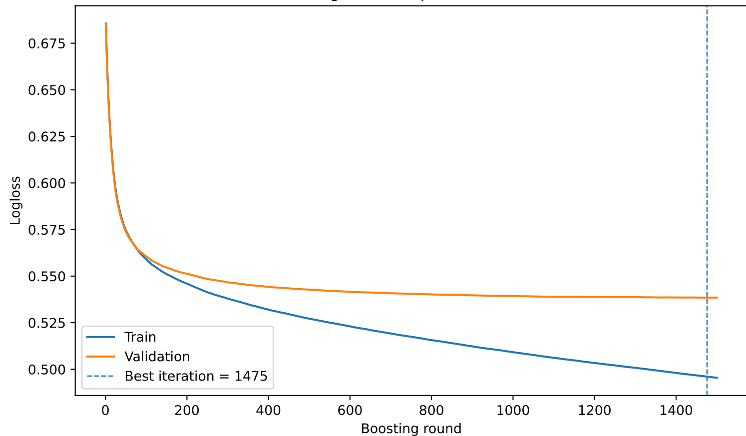
Learning curve: depth=4, child=30
