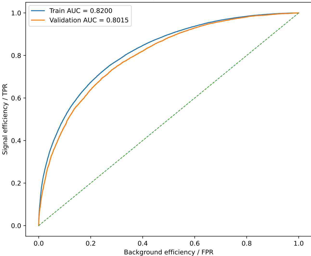
ROC: depth=3, child=30
