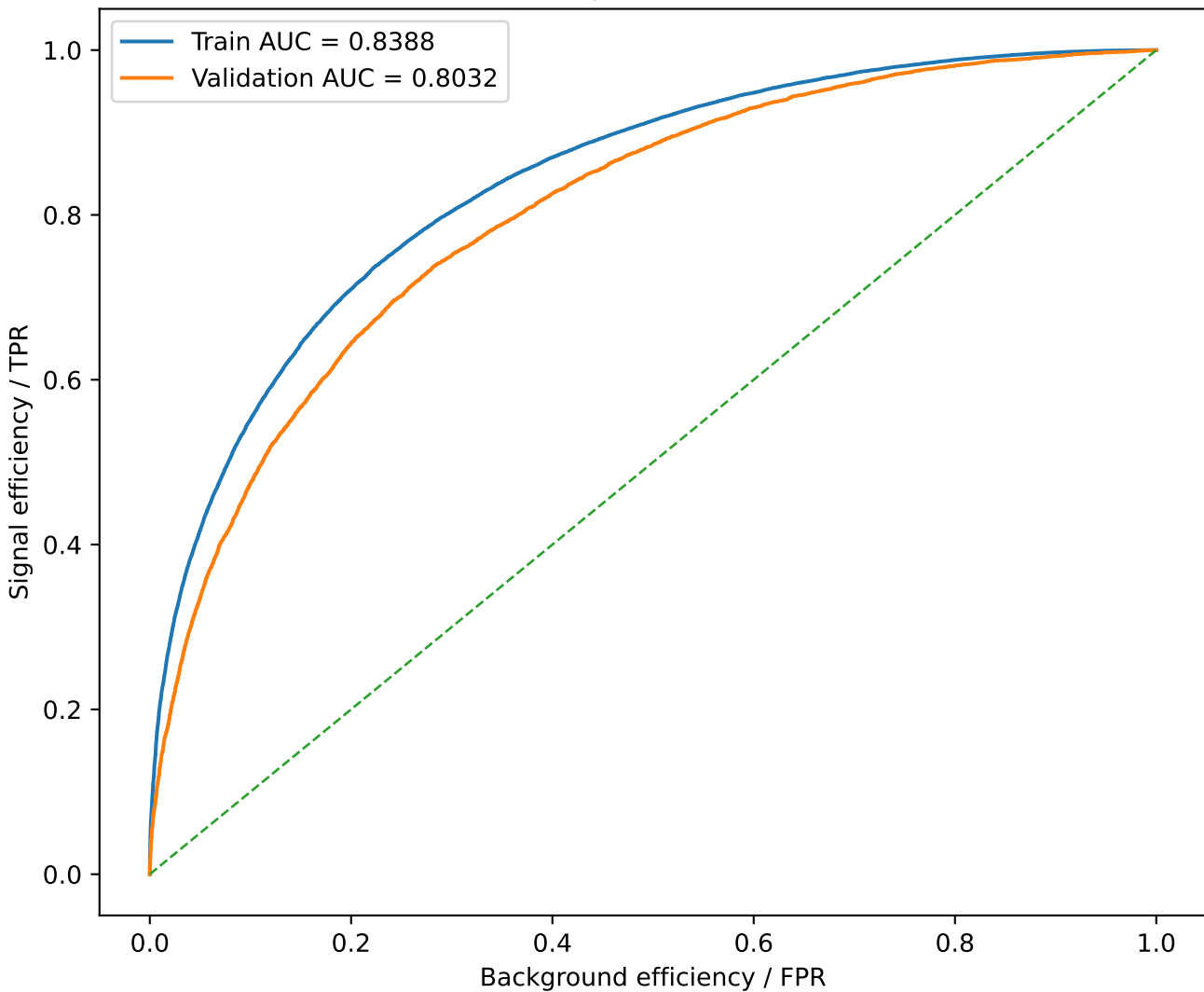
ROC: depth=4, child=10
