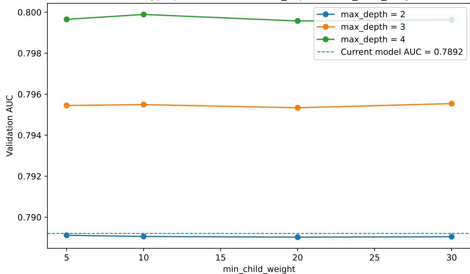
XGBoost hyperparameter scan: max_depth vs min_child_weight
