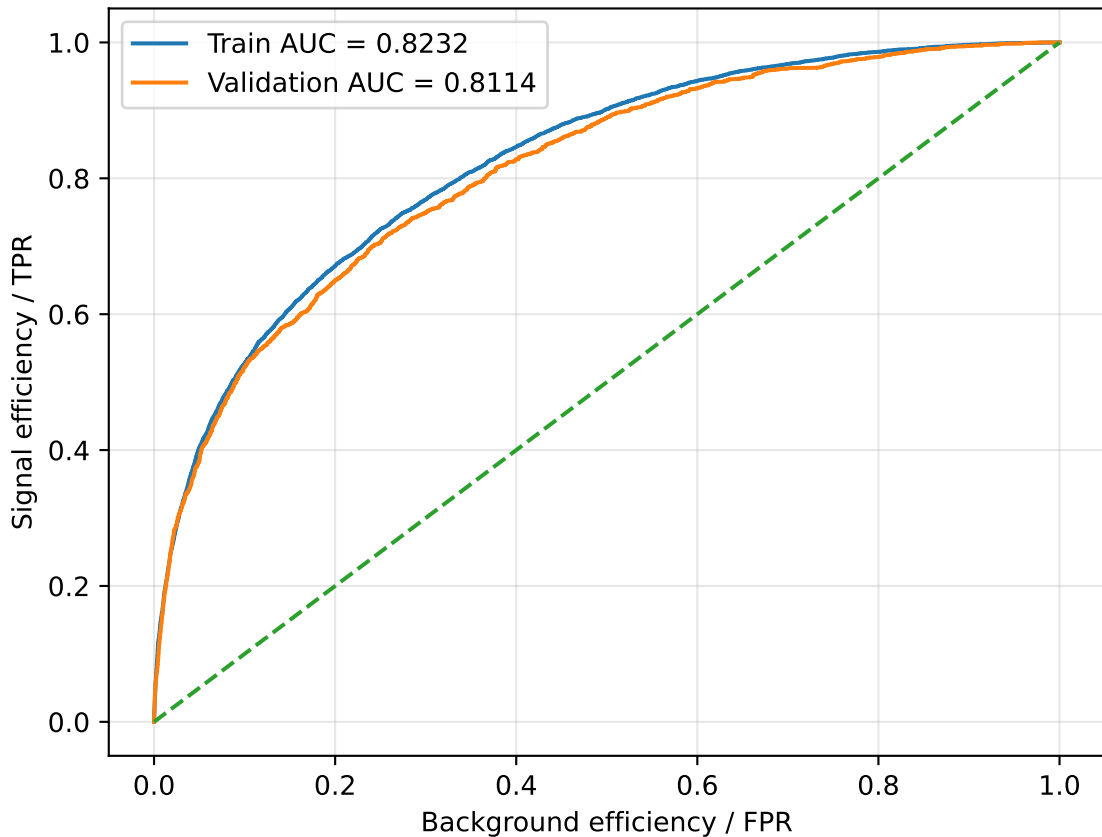
ROC: train vs validation AUC gap = 0.0118
