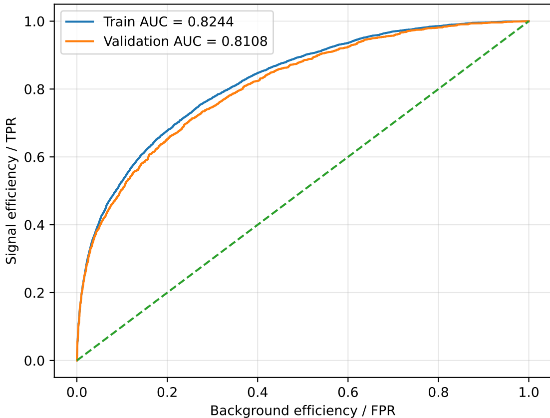
ROC: train vs validation AUC gap = 0.0136
