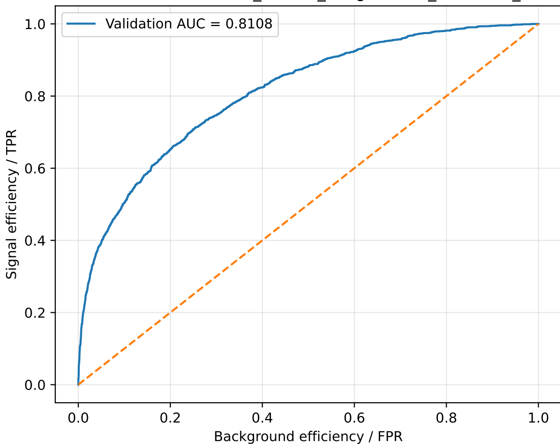
Validation ROC: MHc130_MA125_nbkg100000_boost500_none
